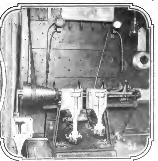
Fig. 21—Method employed of testing the lubricating oil pumps at various speeds by means of a belt and step pulleys
